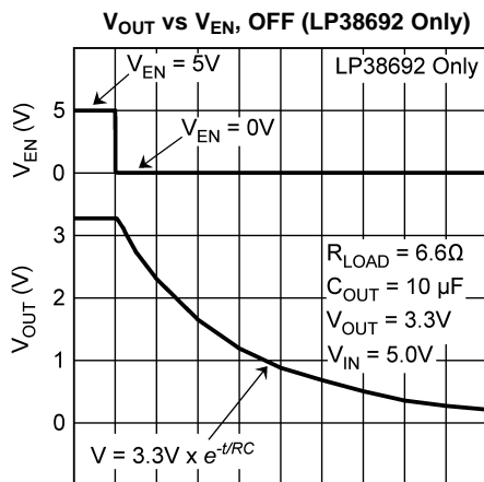
20 \mu\text{s}/\text{DIV} Figure 28.
