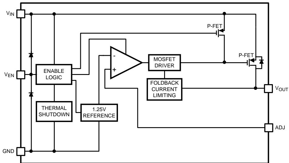
Figure 5. LP38692-ADJ Functional Diagram (SOT-223, WSN)
